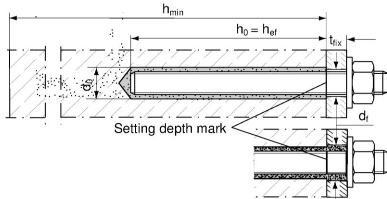
Anchor rod Pre-positioned anchor
